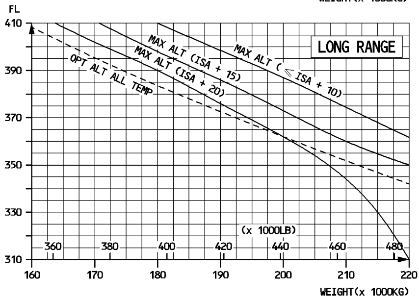
Figure F16: Maximum and Optimum Altitude
