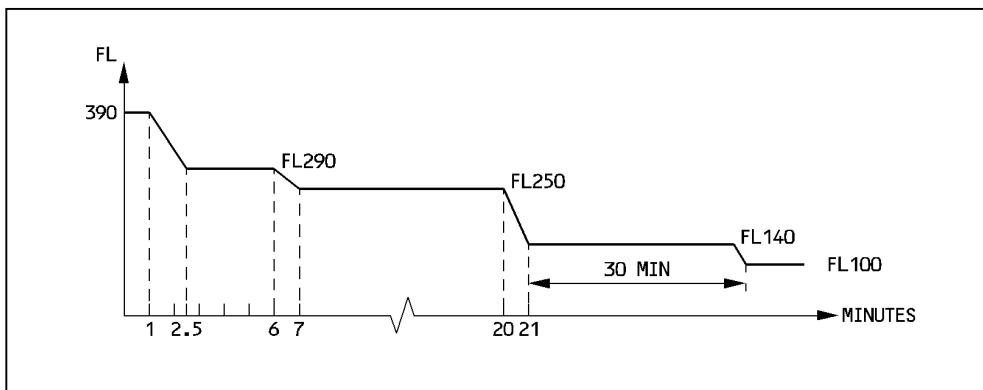
Figure D13: A319 Descent Profile - 22 Minute Oxygen System
